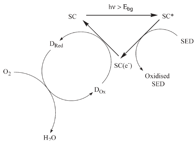
Fig. 6 Schematic illustration of the basic processes associated with a UV-activated oxygen indicator, used to generate the data in Fig. 5, which has the following generic formulation: semiconductor (SC), sacrificial electron donor (SED), redox indicator (initial, highly coloured oxidised form: \text{D}_{\text{Ox}} , photo reduced, usually bleached, reduced form: \text{D}_{\text{Red}} ).
