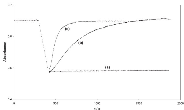
Fig. 5 Typical absorbance (at 610 nm) versus time profiles for a typical UV-activated oxygen indicator, recorded under the following different gaseous environments: (a) \text{N}_2 , (b) air and (c) oxygen. Each film was initially left to stand for 3 minutes, before being exposed to a short burst (2.5 min) of UVA light (provided by a 100 W BLB), to activate, i.e. bleach, the film (broken line). The subsequent recovery of the original colour/absorbance of the indicator film then depended upon the percentage \text{O}_2 in the ambient gas phase. 28
