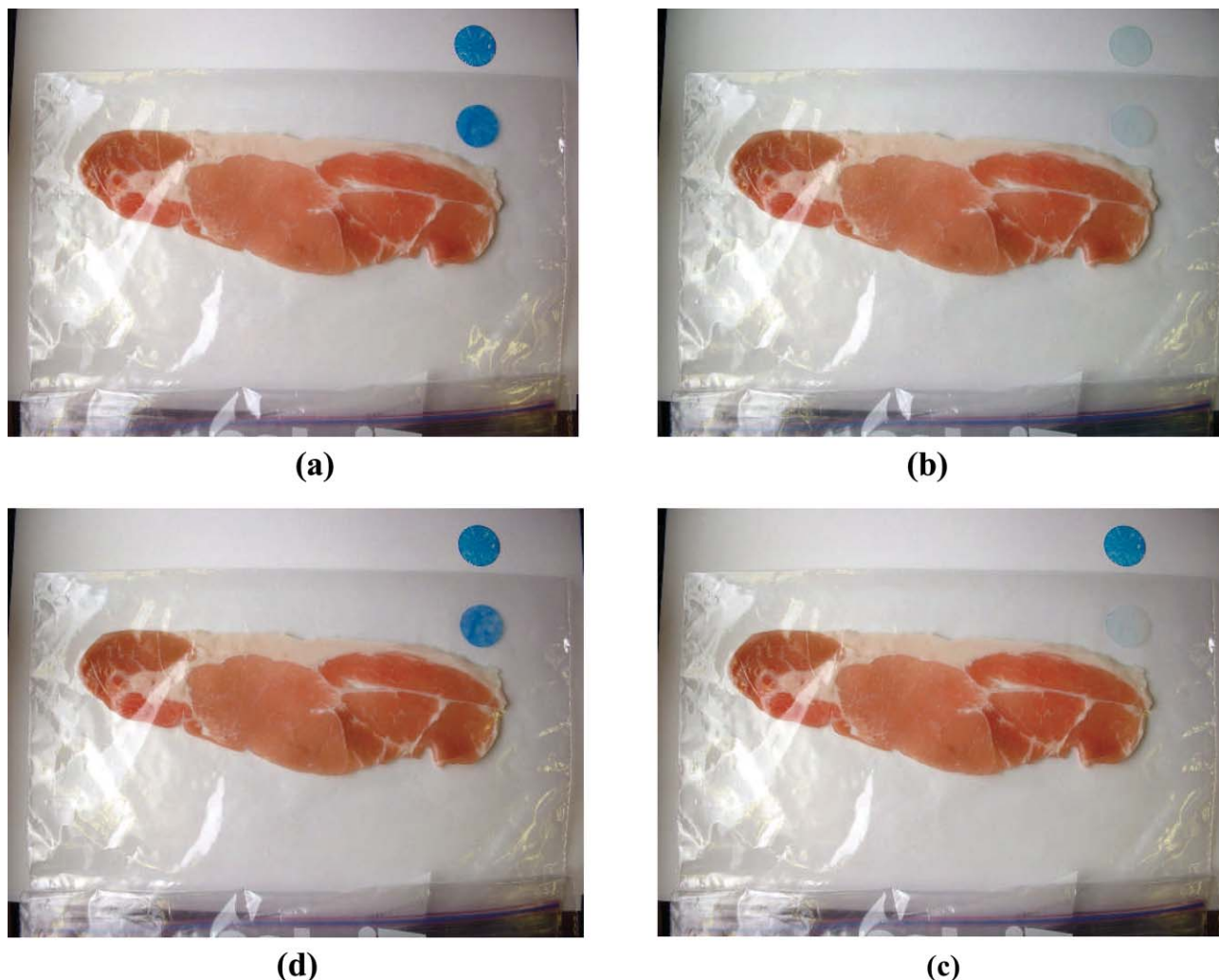
Fig. 7 Photographs of two typical blue-coloured UV-activated oxygen indicators with the formulation: MB/TiO 2 /TEOA/HEC, one placed inside and the other outside a plastic package flushed with CO 2 and sealed. In (a) the package had just been sealed and the two indicators are blue. The two indicators were then bleached by a short (2.5 min) burst of UVA light (b). The indicator outside the package regained its original colour within minutes, whereas, 48 h later, the indicator inside remained bleached (c). Finally, upon opening the package, the indicator within regained its original colour in response to the ingress of oxygen (d).
