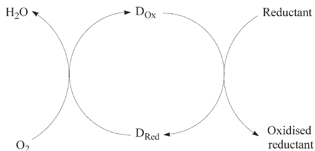
Fig. 3 Schematic illustration of the basic processes associated with a colorimetric redox dye-based oxygen indicator, where \text{D}_{\text{Ox}} and \text{D}_{\text{Red}} are the oxidised (usually highly coloured) and reduced (usually bleached) forms of the redox dye, respectively. The reductant is usually a reducing sugar in alkali, metal ion (often \text{Fe}^{2+} ) or ascorbic acid.
