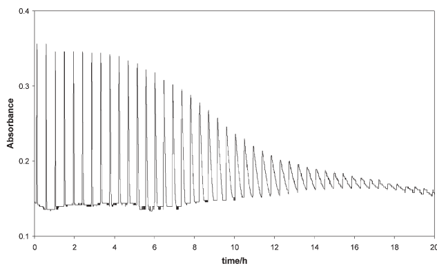
Fig. 4 Typical absorbance (at 640 nm) versus time profiles for a dichloroindophenol/fructose/tetrabutyl ammonium hydroxide/ethyl cellulose oxygen indicator film exposed to a cycle of air (high absorbance) for 1 min and nitrogen (low absorbance) for 25 min over a period of 20 h. Note: within 10 min in air the response features of the oxygen indicator film begin to change markedly. 22
