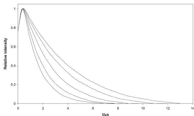
Fig. 2 Typical relative fluorescence intensity versus time profiles for an OxySense ™ O 2 xyDot ™ exposed to different O 2 –N 2 gas mixtures. The percentage O 2 in these mixtures was (from slowest to fastest decay): 0, 2.1, 6.3, 12.6 and 21.0%, respectively. 13
